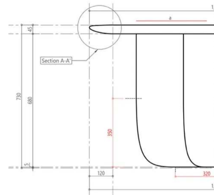
2 ENWA - MARU DINING TABLE 1300 - FRONT ELEVATION TABLE 1:10
