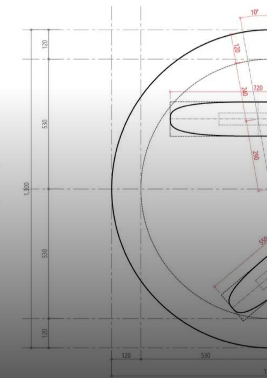
3 ENWA - MARU DINING TABLE 1300 - PLAN TABLE 1:10
